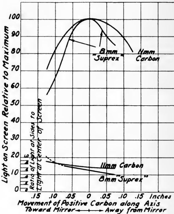
FIG. 4. Curves showing the change in total screen light and the distribution of screen light with movement of positive carbon, for the 8-mm "Suprex" and the 11-mm carbon used with their respective optical systems.
